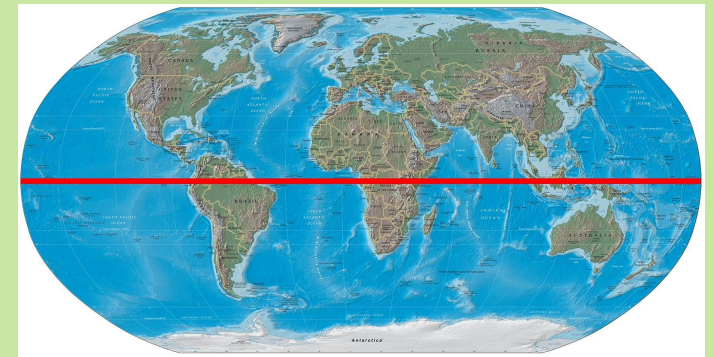
The red line shows the equator, which separates the top of the Earth and the bottom.
